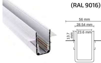
Trimless Magnet Ray / Trimless Magnetic Track
