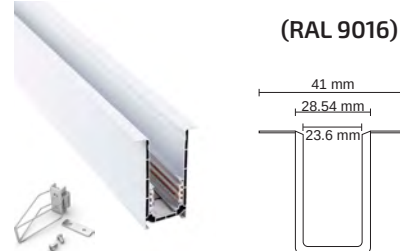
Siva Altı Yaylı Magnet Ray / Recessed Spring Magnetic Track
