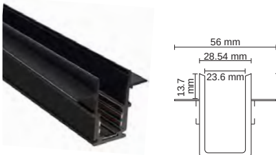
Pc Trimless Magnet Ray / Pc Trimless Magnetic Track
